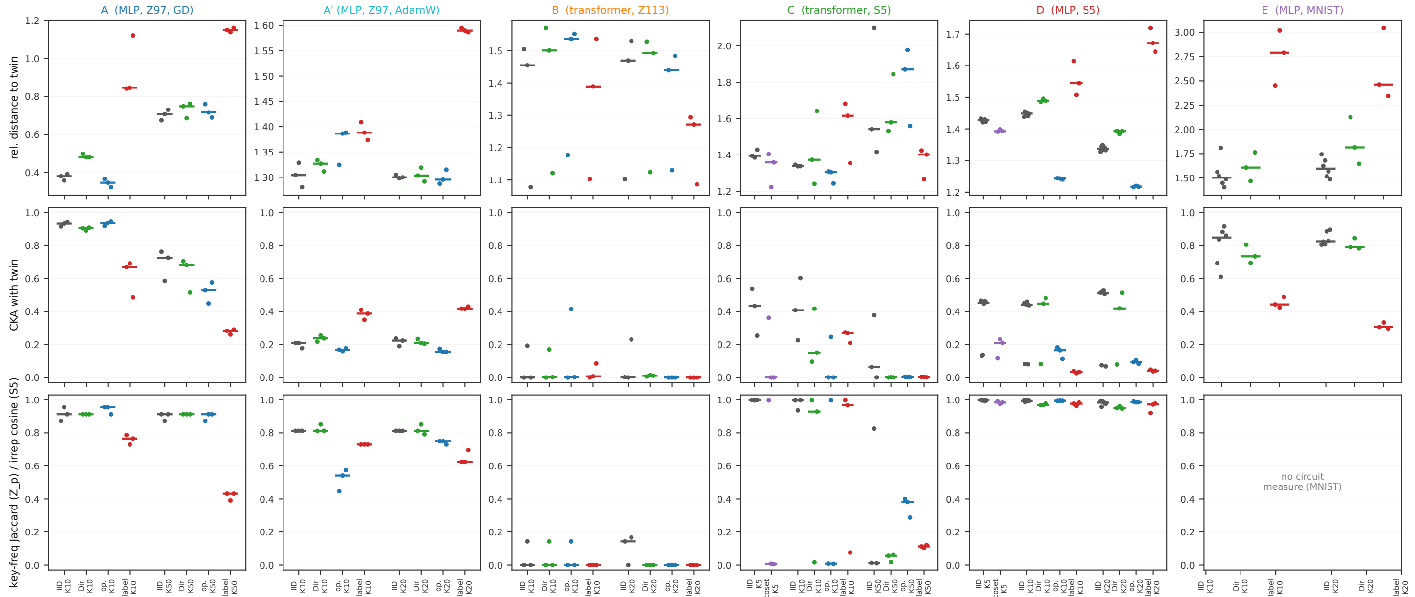
Twin similarity at the end by data partition: incoherent (label) shards move GD furthest from the centralised solution
