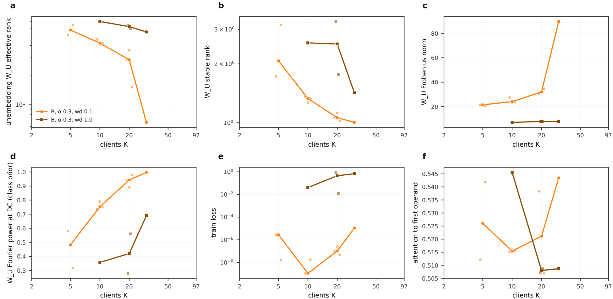
Setup B at first crossing: high-K transformers generalise with an unembedding collapsed onto the class-prior direction
