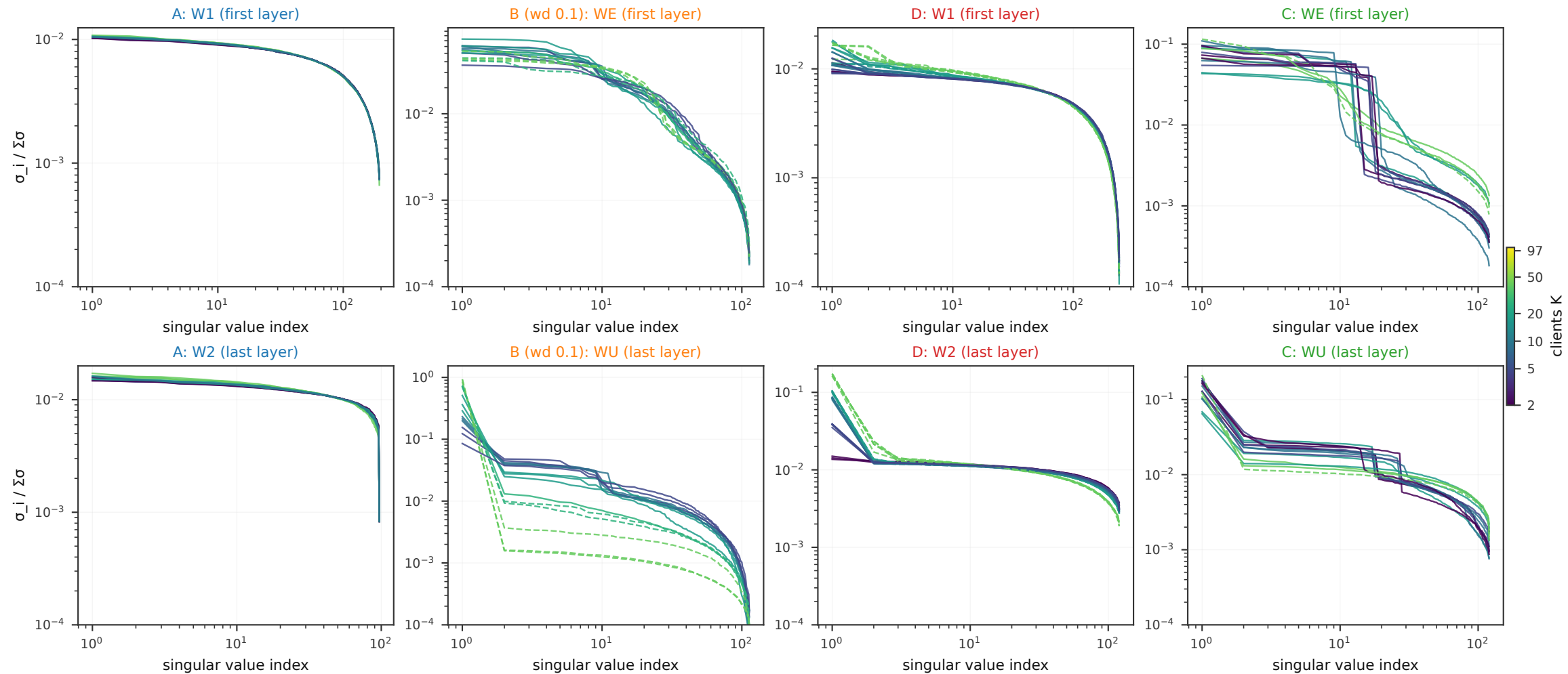
Singular-value spectra at first crossing (dashed: never crossed, last checkpoint), coloured by K
