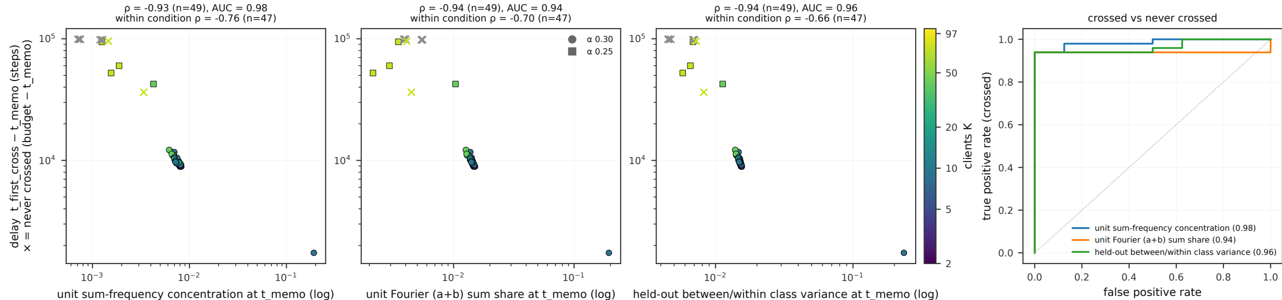
Setup A: sum-frequency structure in the hidden units at memorisation separates slow from fast conditions (colour: K; square: \alpha 0.25), and still ranks runs within a condition
