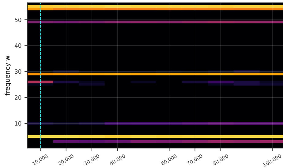
B (transformer, Z113), K = 20, seed 42
