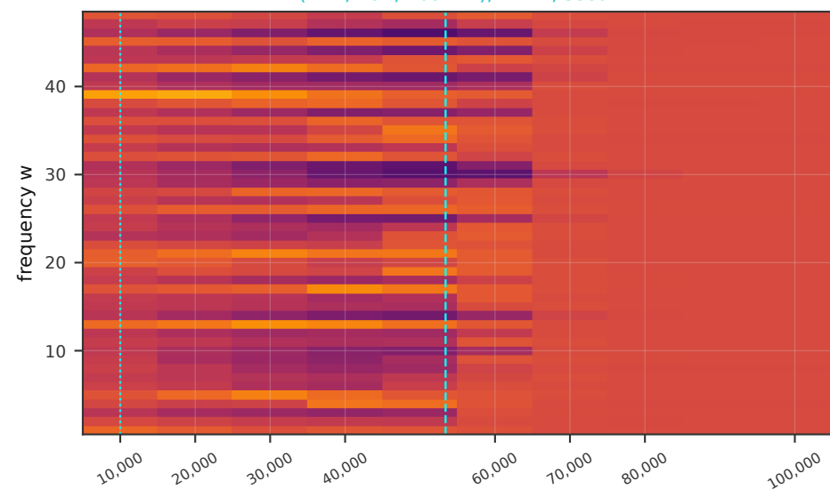
B (transformer, Z113), K = 2, seed 42
