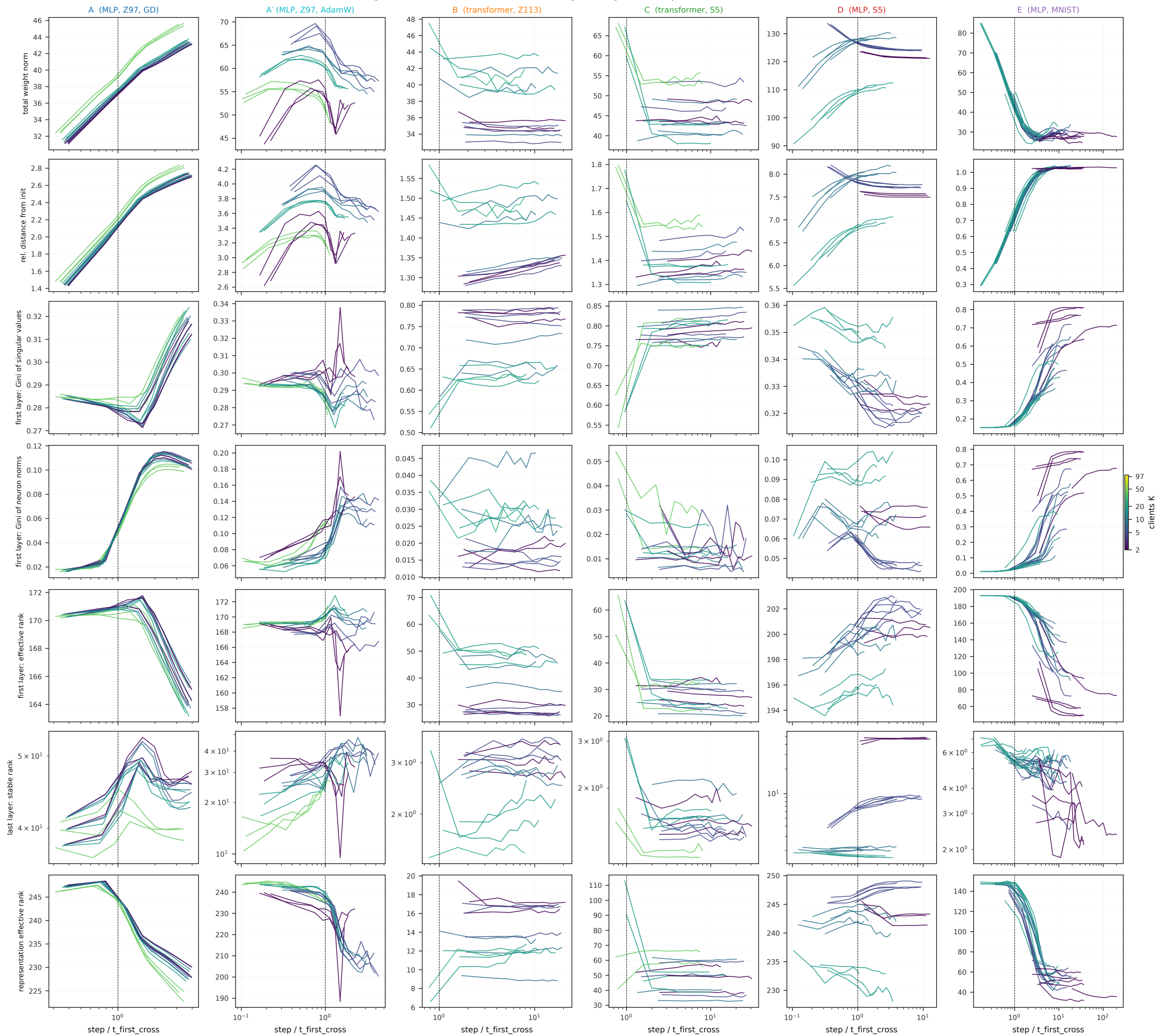
Weight norms, Gini coefficients and ranks through training, coloured by K (IID ladders; crossed runs)
