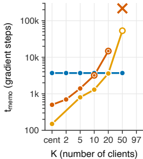
(b) Time to memorise vs K
