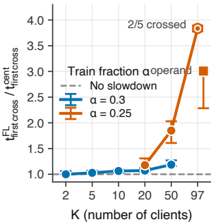
(a) Slowdown vs K (setup A, IID)
