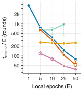
(b) Memorisation rounds vs E
