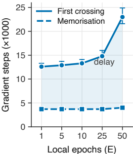
(a) Grokking time vs E (setup A)
