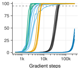
(b) H1: \alpha=0.25 , E=25, IID
