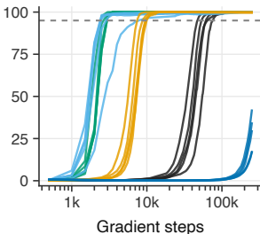
(c) H2: \alpha=0.25 , E=25, non-IID
