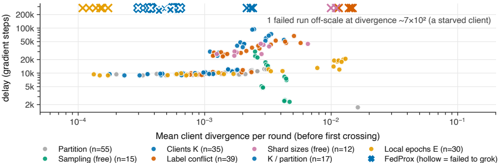
(a) Delay vs client divergence (setup A, FedAvg, every design axis)
