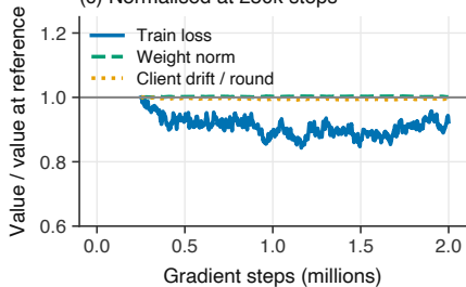
(c) Normalised at 250k steps
