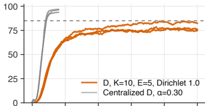
(b) Test accuracy, Dirichlet 1.0
