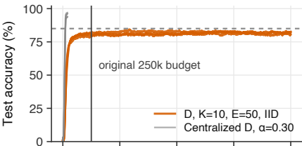
(a) Test accuracy, E=50 , 2M steps
