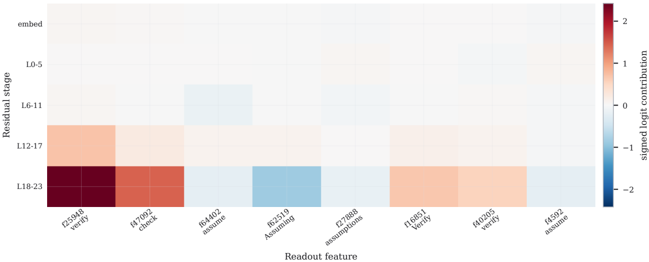
Qwen3.5-2B 32x Prism-DLA: verify - assume
