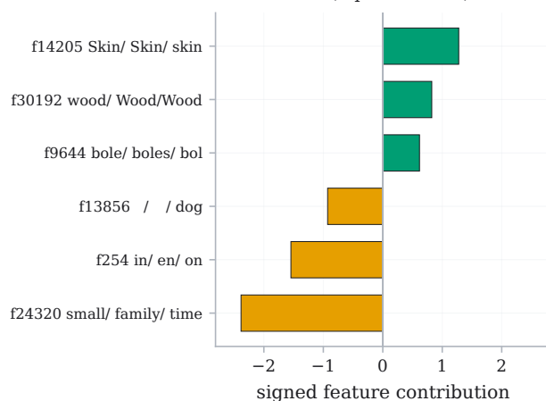
C Tree context: bark - dog exact +10.94; sparse +6.59; resid +4.35
