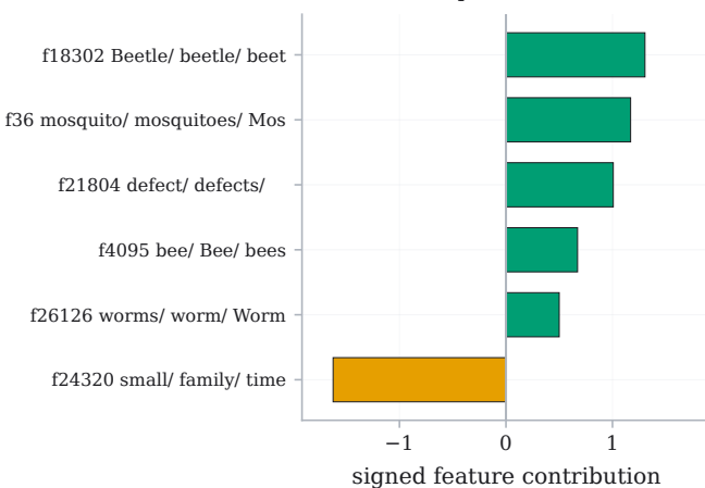
C Tree context: bark - dog exact +10.94; sparse +6.59; resid +4.35
