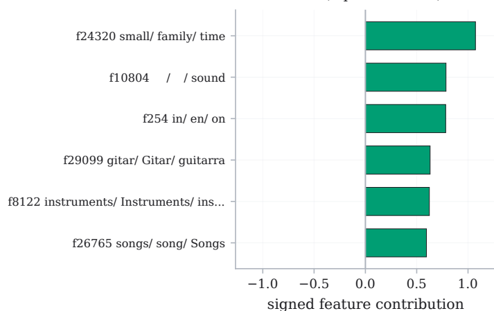
D Music context: bass - trout exact +12.97; sparse +12.42; resid +0.54
