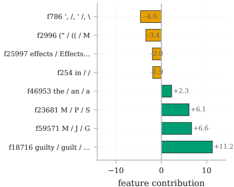
B Selection pressure: Winner vs rank-5 competitor exact +3.6; sparse +3.5; rho 0.04
