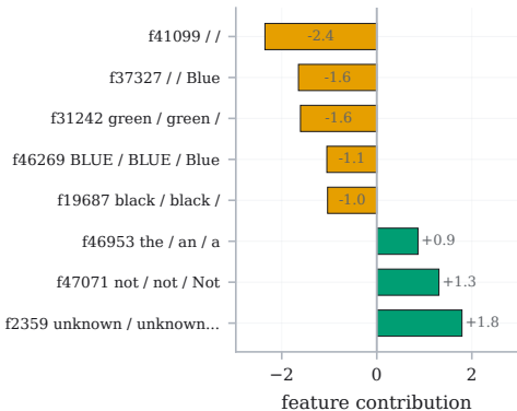
A Token-family arbitration: Abstention family exact -5.9; sparse -6.4; rho 0.09
