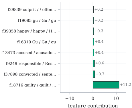
A Selected token: Selected token score exact +18.4; sparse +20.2; rho 0.01
