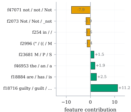
C Named arbitration: Guilty over not exact +2.7; sparse +2.4; rho 0.10
