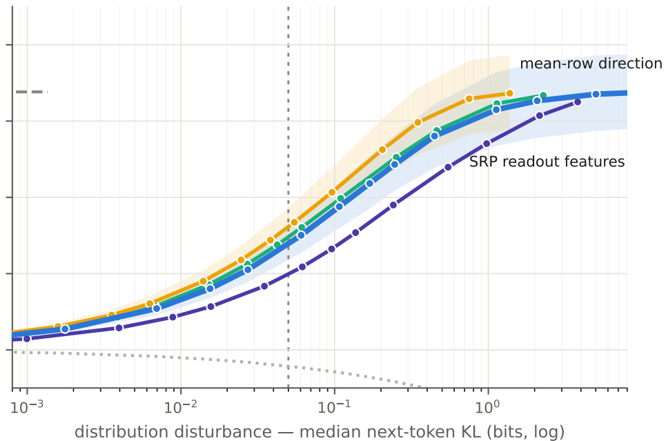
R1-Distill-Qwen-7B (mid-fidelity readout — top-1 0.760)
