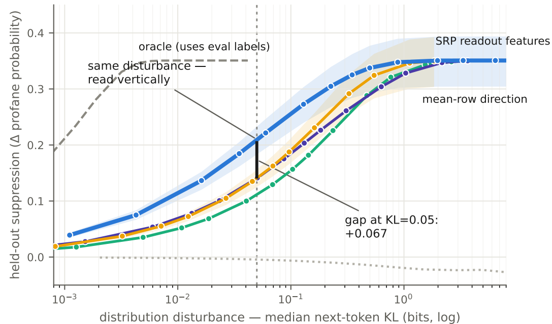
Qwen3.5-2B (display model — replacement top-1 0.887)
