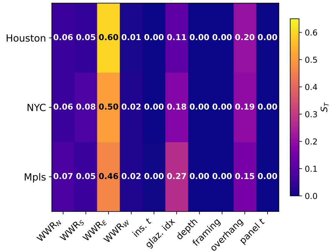
(b) Path-B Sobol S_T on annual EUI (ISO 13790) (climate-dependent)
