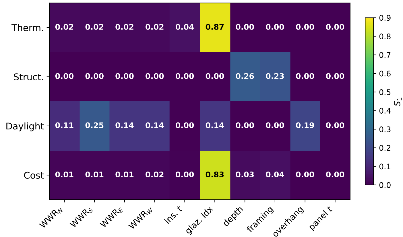
(a) Path-A Sobol S_1 on analytical objectives (climate-invariant by construction)
