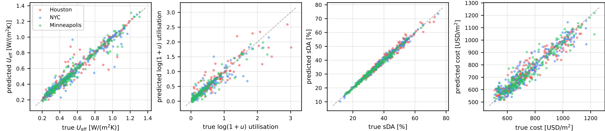
Gaussian-process surrogate accuracy (5-fold CV) across four objectives and three cases
