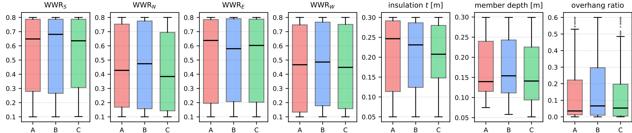
Design-variable distributions across Pareto-optimal designs (A: Houston, B: NYC, C: Minneapolis)
