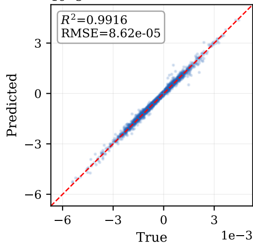
C_m (Pitch moment)
