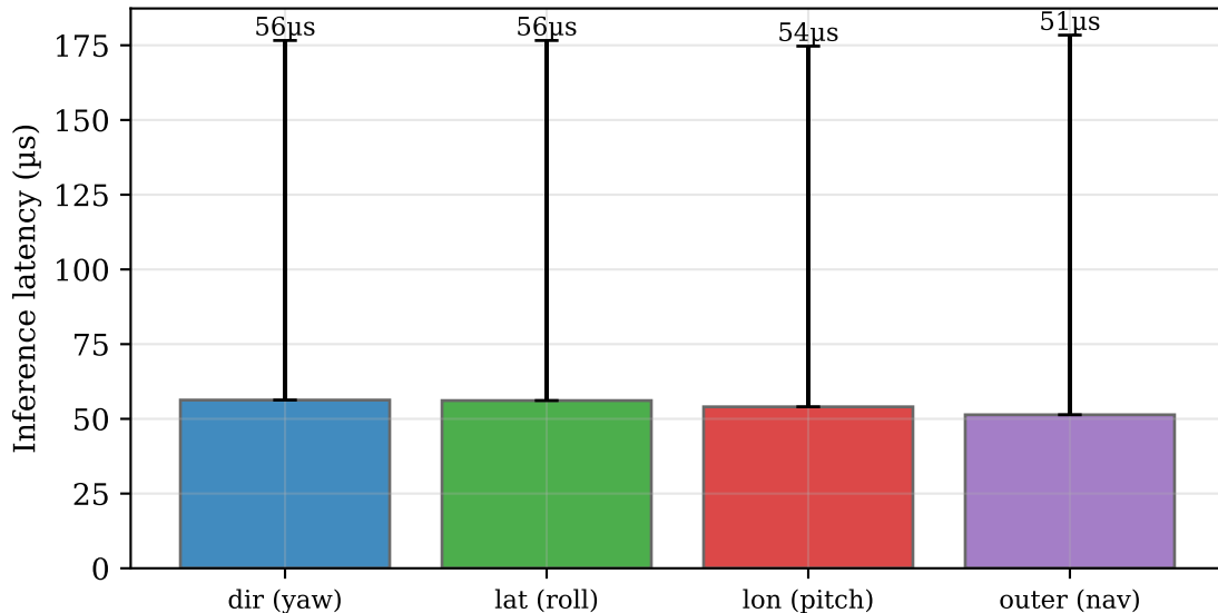
Per-network single-step inference latency (CPU, 1 thread; bar=mean, whisker=p99)
