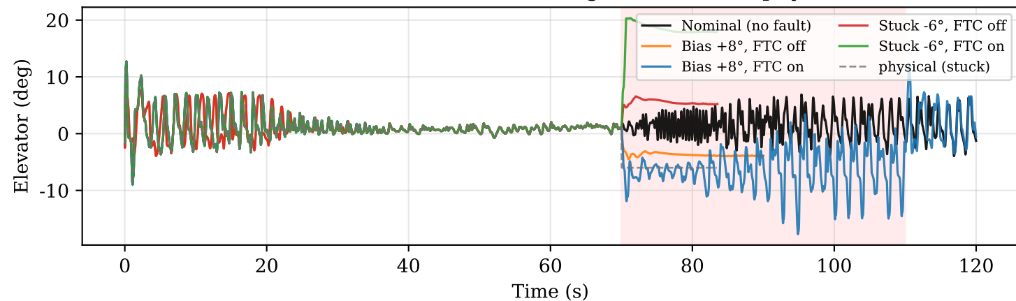
(c) Commanded elevator (solid; FTC augmentation) vs physical (dashed)
