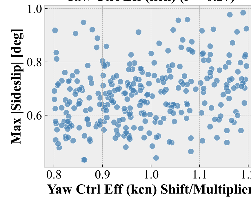
Yaw Ctrl Eff (kcn) ( r=+0.27 )
