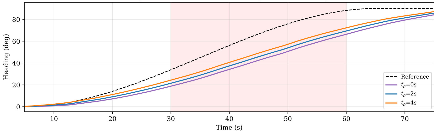
(d) Heading trace (fault window shaded): preview reduces phase lag
