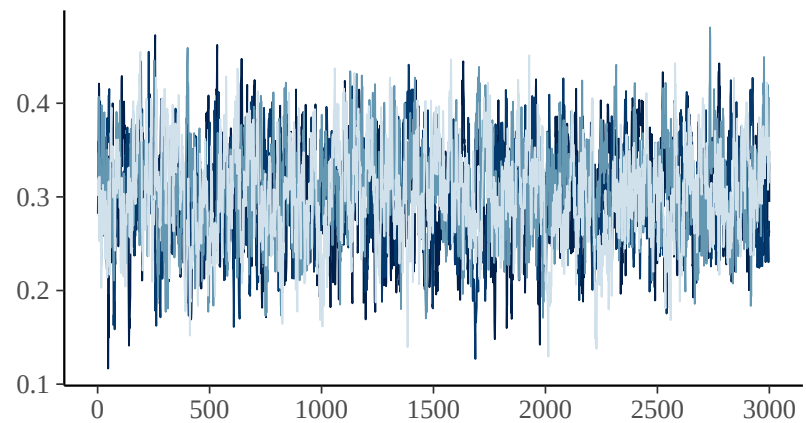
b_feature_setTSFEL
