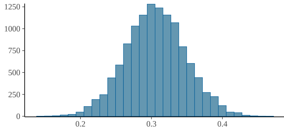
b_feature_settsfeatures
