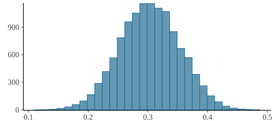
b_feature_setTSFEL
