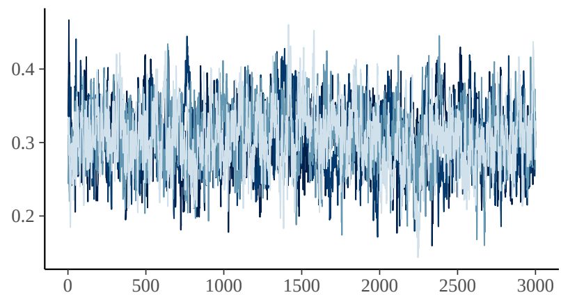
b_feature_settsfeatures
