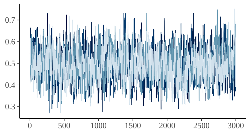
b_feature_settsfresh
