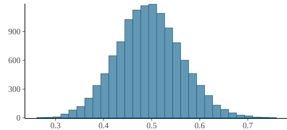
b_feature_settsfresh
