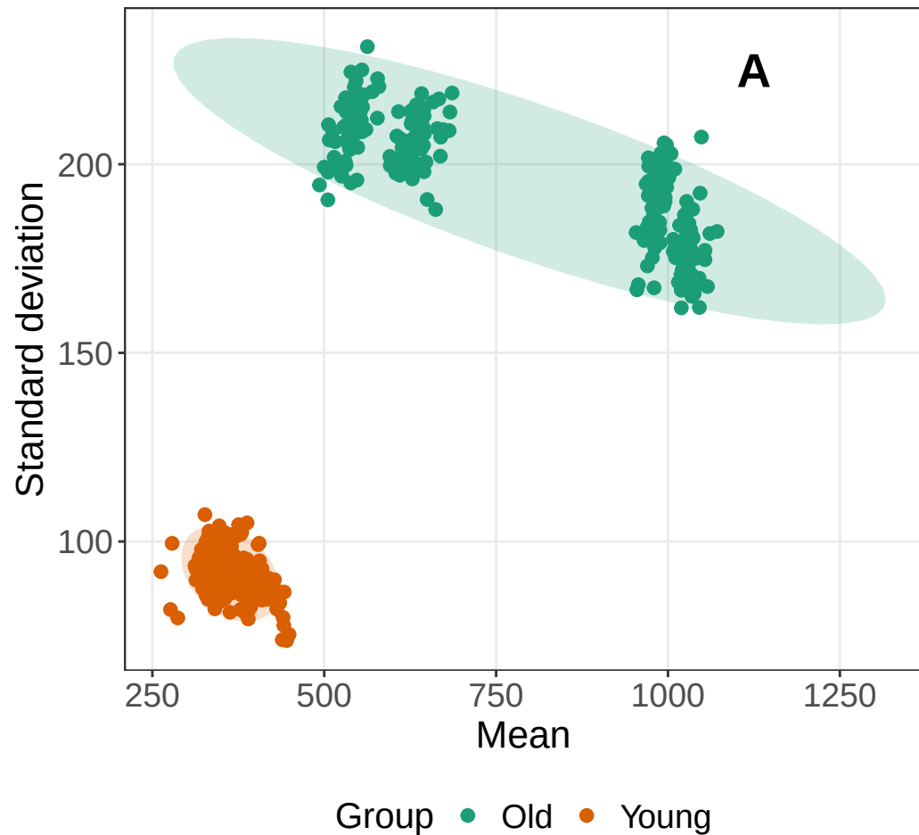
GunPointOldVersusYoung
