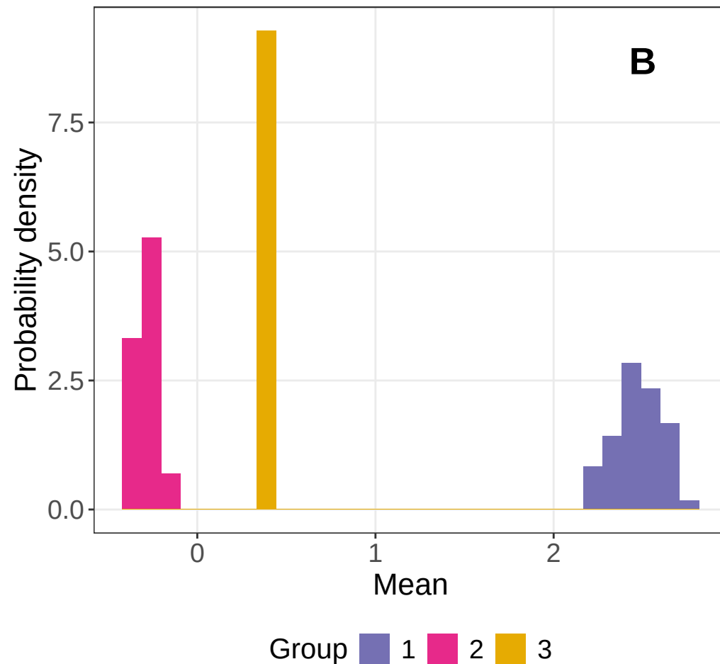
InsectEPGRegularTrain
