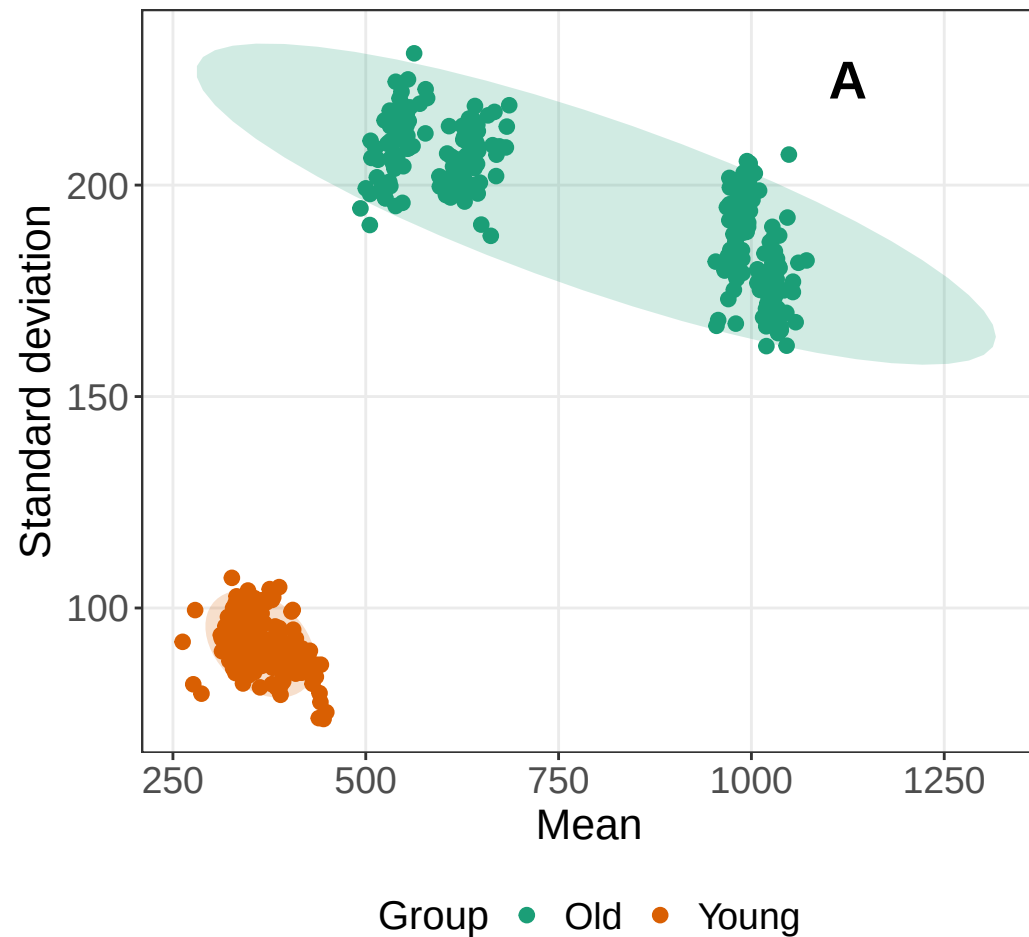
GunPointOldVersusYoung
