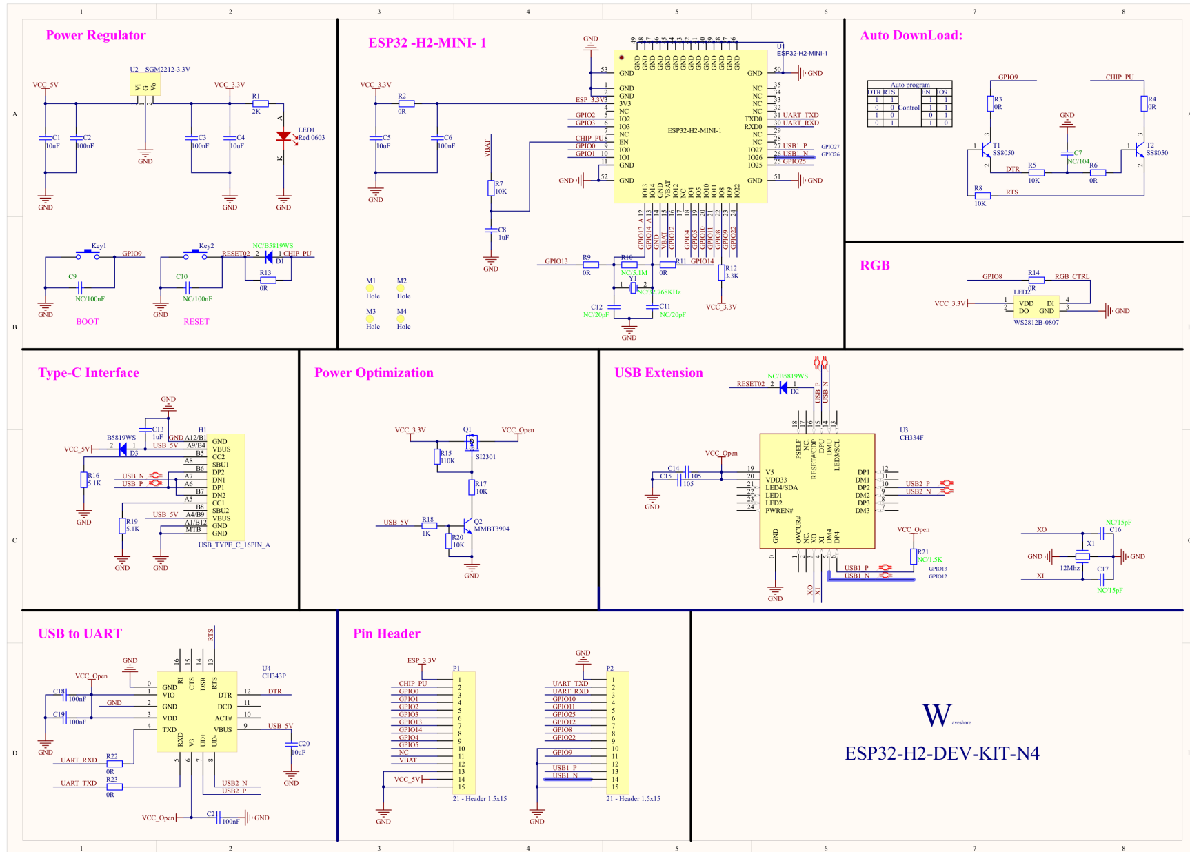
Gambar B.1: Skematik Waveshare ESP32-H2-DEV-KIT-N4
