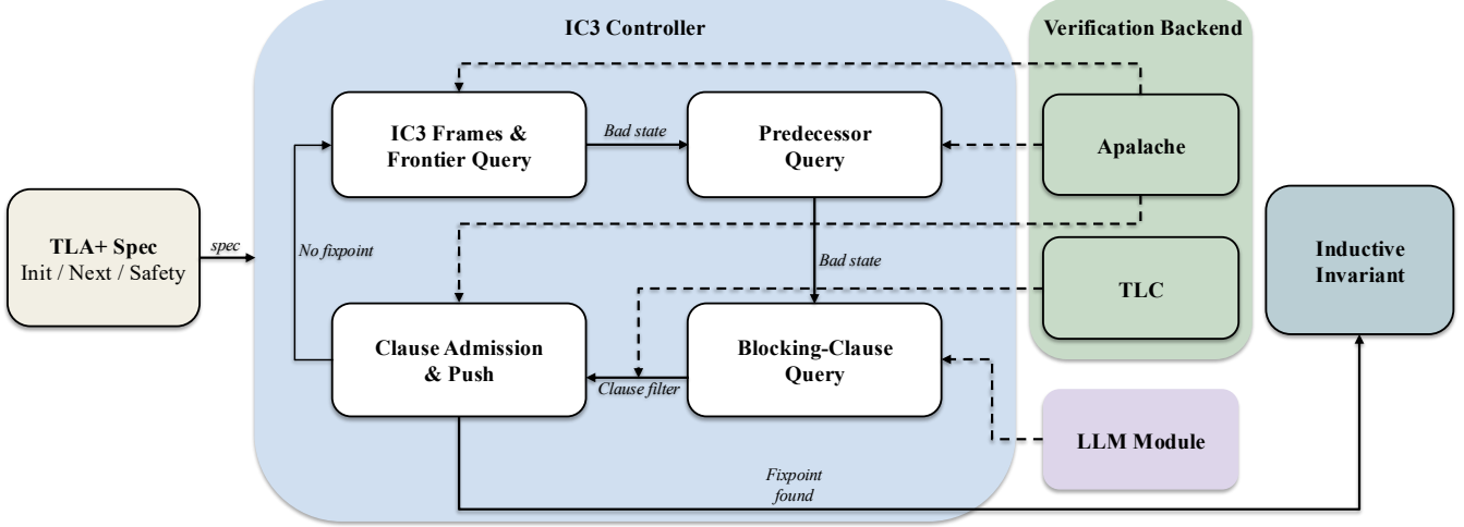
Figure 1. Overview of IC3Syn. The IC3 loop iterates through four stages: frontier query, backward predecessor search, blocking-clause search, and clause push. They are coordinated by three components: (1) an IC3 controller that maintains frames and manages backward search from frontier bad states, (2) a verification backend where Apalache handles symbolic witness queries and TLC screens candidate blocking clauses against concrete reachable states, and (3) an LLM module that proposes candidate blocking clauses from protocol context and representative bad states.
