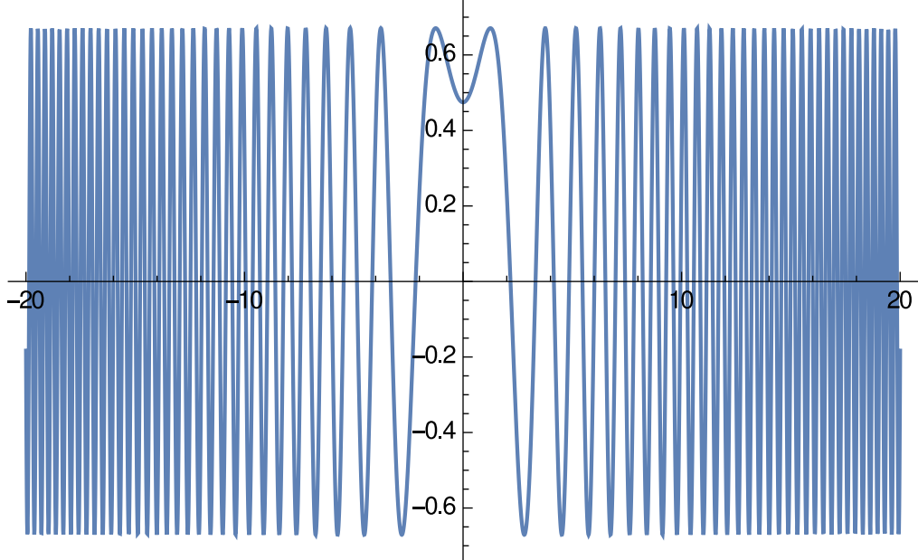
D(x,0,\pi/4) without cutoff
