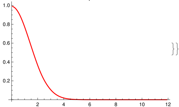
timestep=1000
