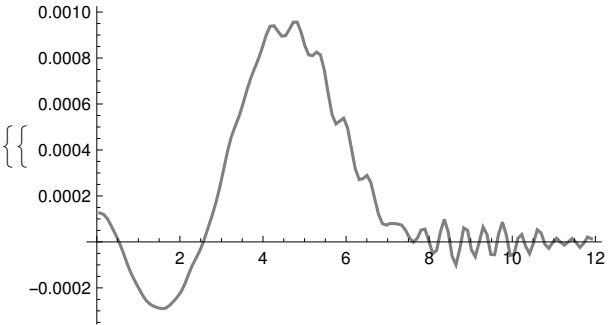
timestep=5000, t=4999.
