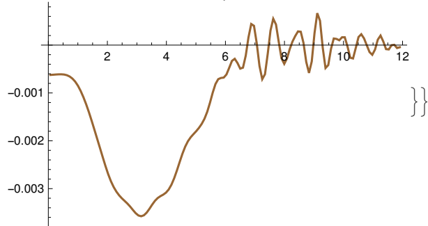
timestep=5000
