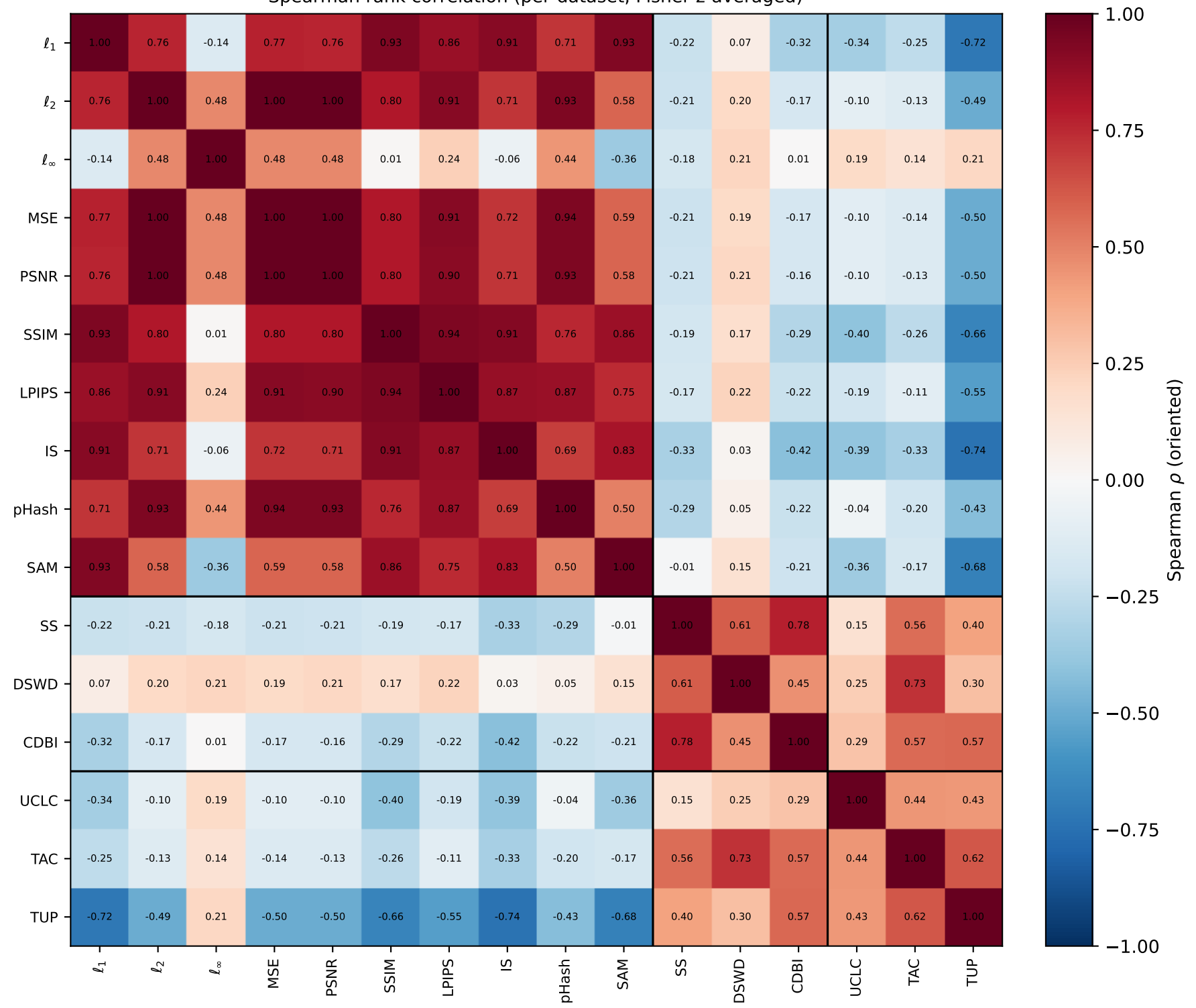
Spearman rank correlation (per-dataset, Fisher-z averaged)
