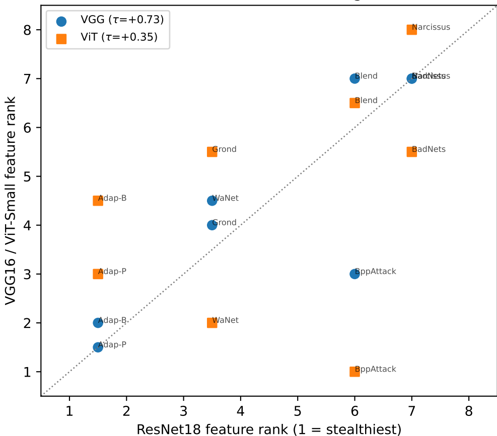
Cross-architecture feature ranking (CIFAR-10)
