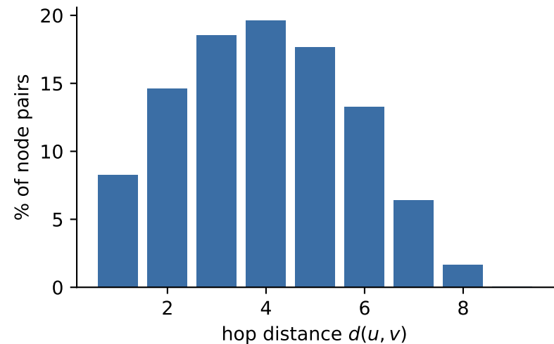
CIFAR10 (mean diam 8.5)
