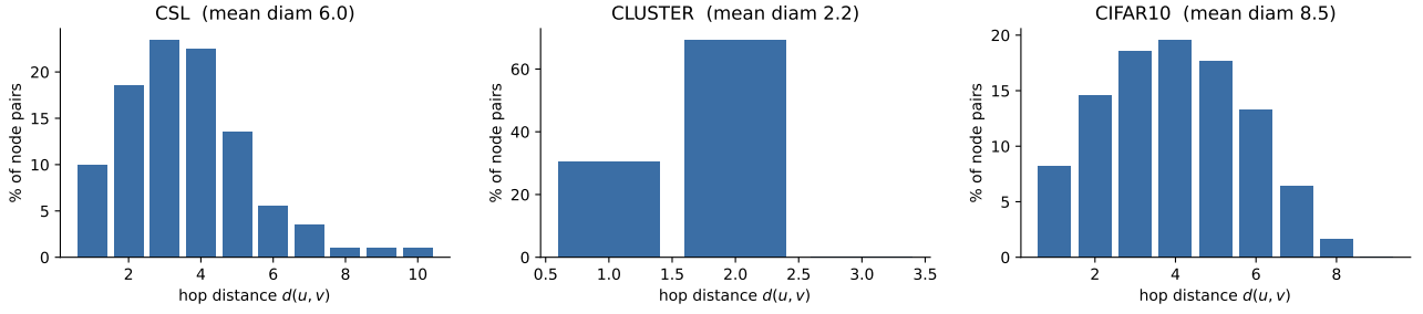
Figure 2: Hop-distance distribution per dataset, measured before training.
