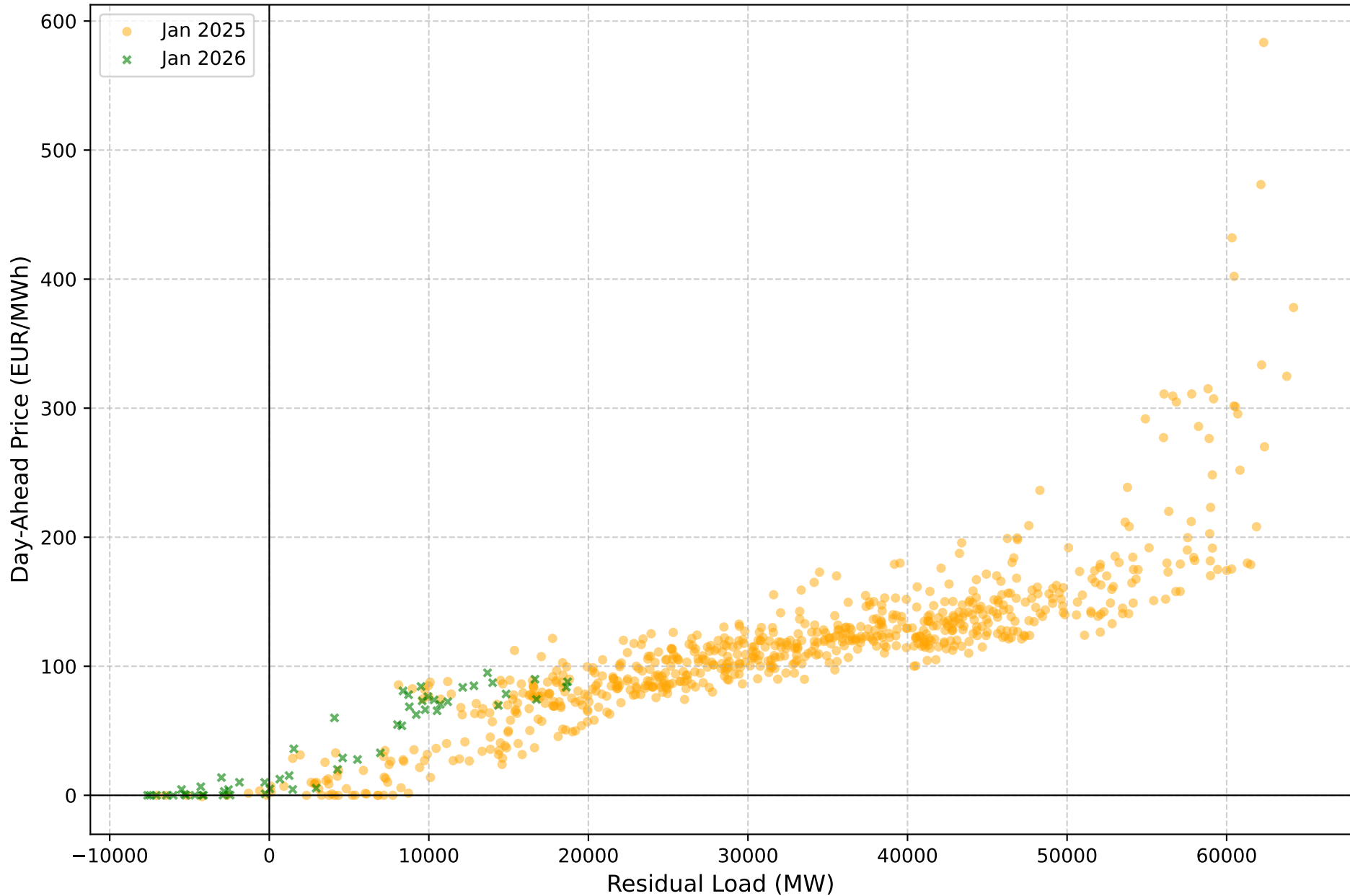
Residual Load vs Price - January 2025 vs 2026
