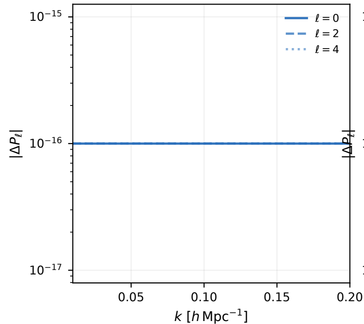
Exchange symmetry
