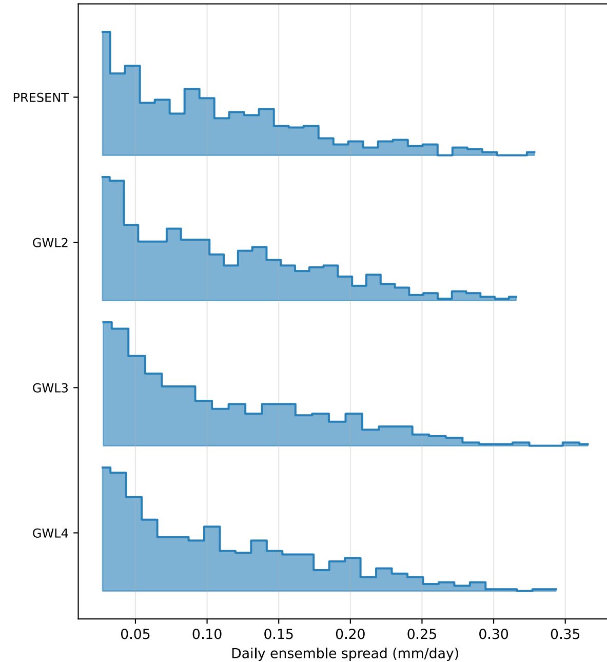
Precipitation
