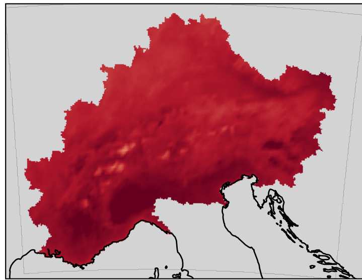
Temperature - Interpolated field
