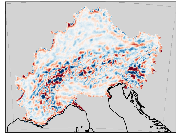
Temperature - Downscaled — interpolated field
