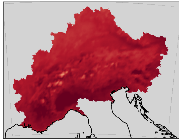
Temperature - Downscaled field
