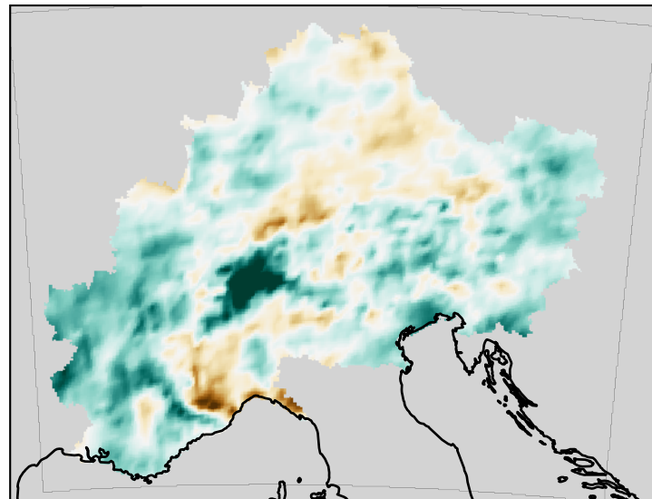
Precipitation - Interpolated field
