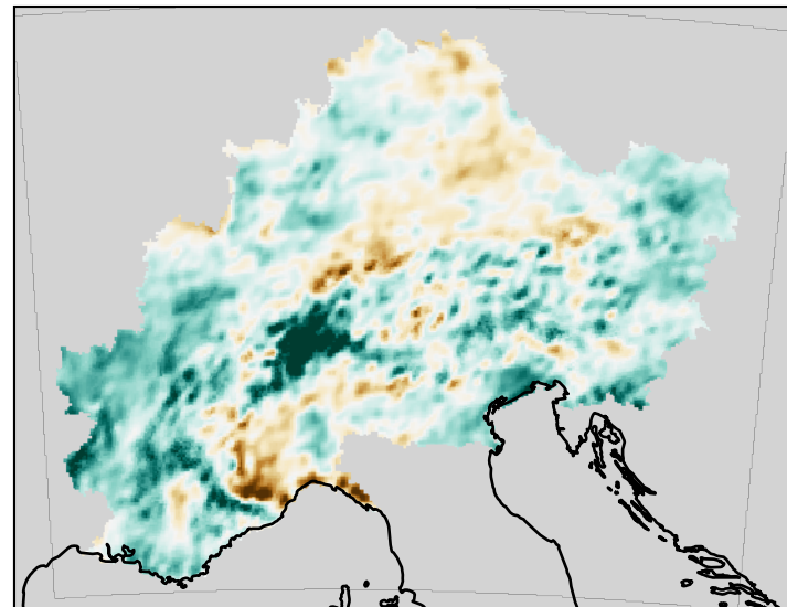
Precipitation - Downscaled field
