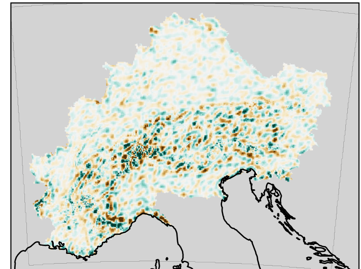
Precipitation - Downscaled — interpolated field
