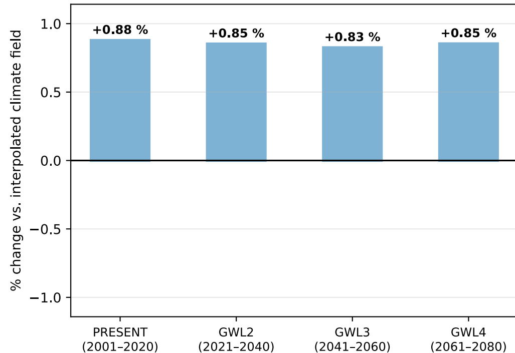
Total precipitation mass
