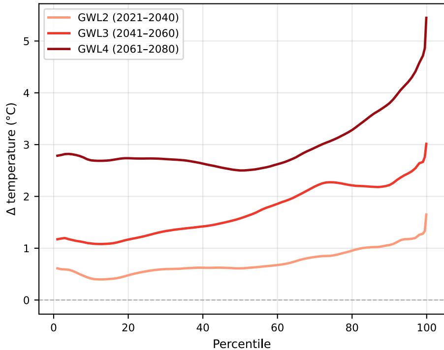
Surface air temperature
