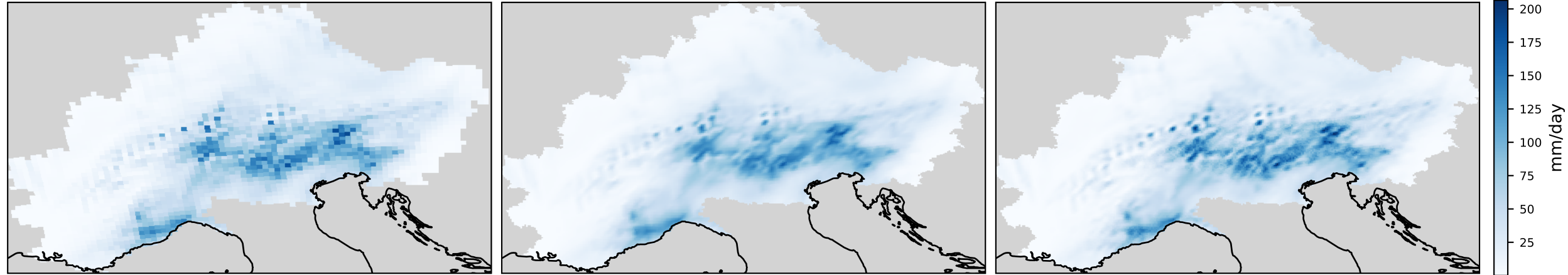
Precipitation - Coarse field
