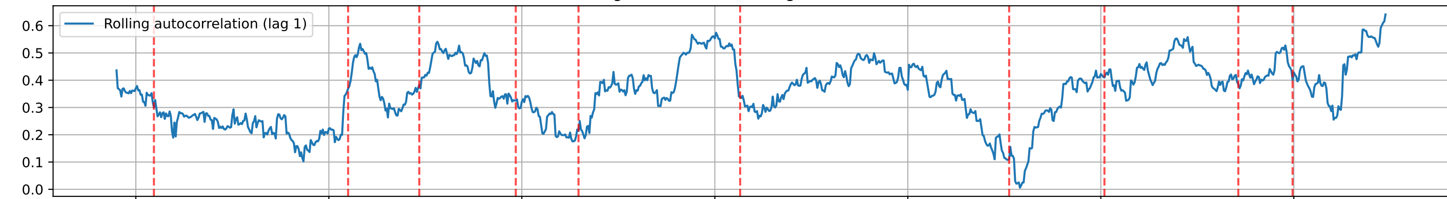
Rolling Autocorrelation (Lag 1) (144 months)
