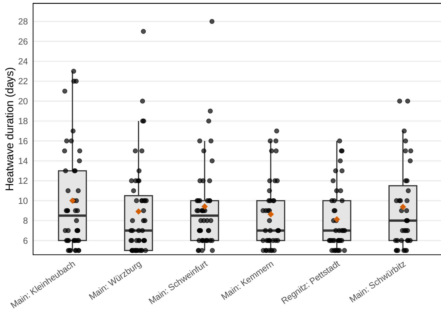
Heatwave duration by station
