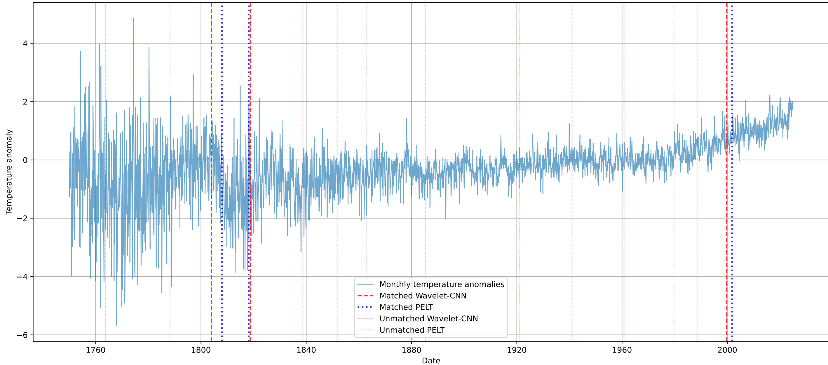
Matched and Unmatched Change Points (Tolerance: \pm 72 Months)
