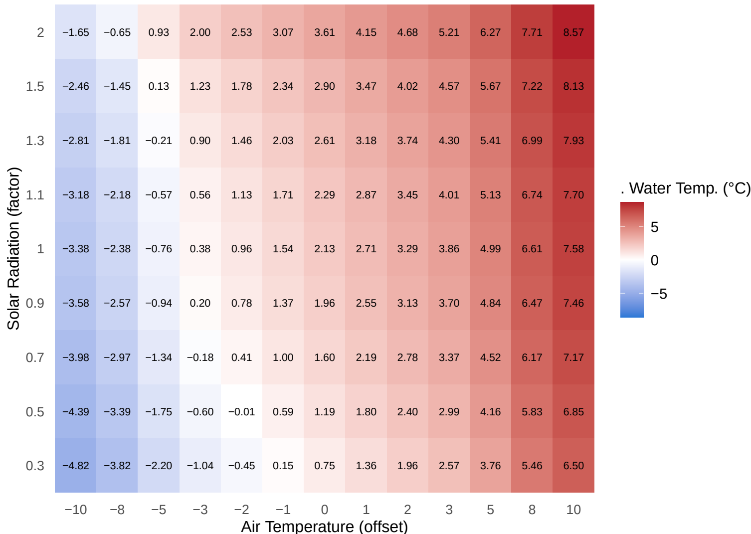
2D Partial Dependence: Air Temperature × Solar Radiation
