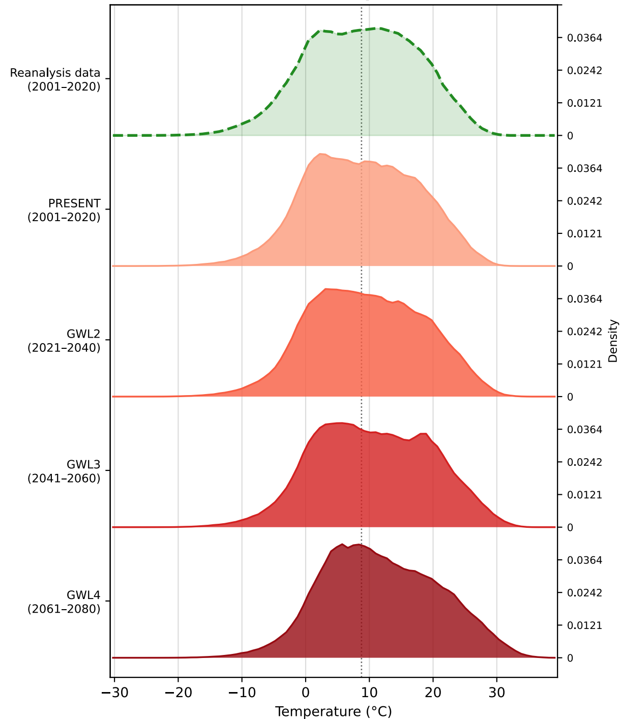
Surface air temperature
