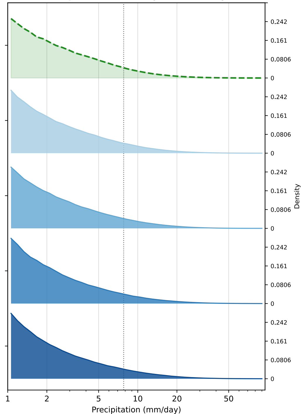
Precipitation (wet days > 1mm/day)
