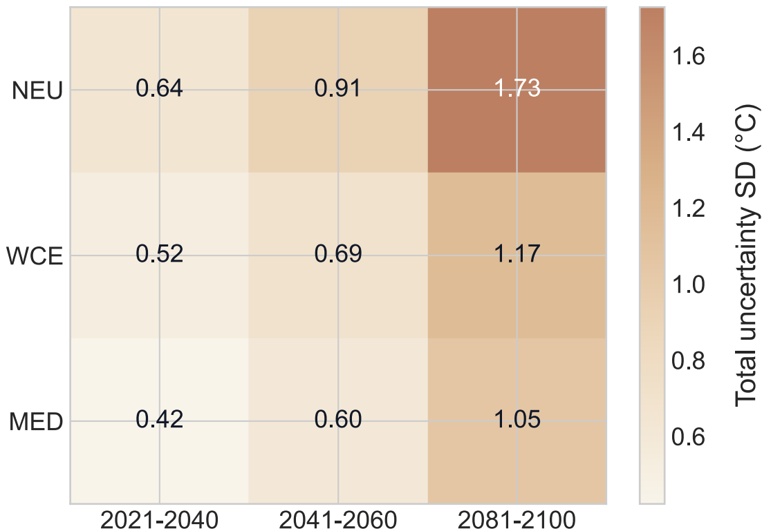
Total uncertainty SD by region and period
