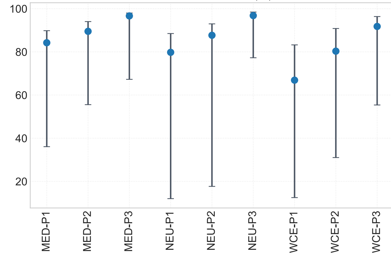
Model contribution (%)
