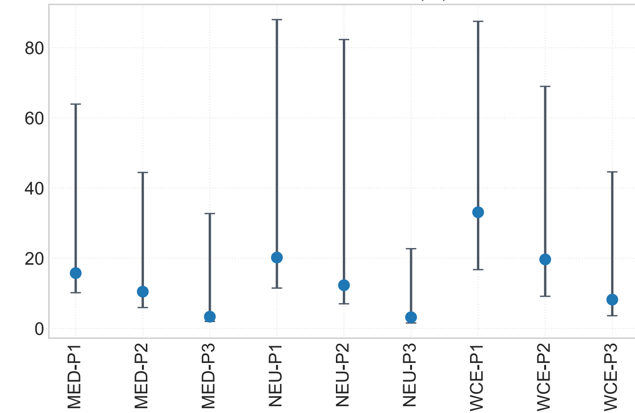
Internal contribution (%)
