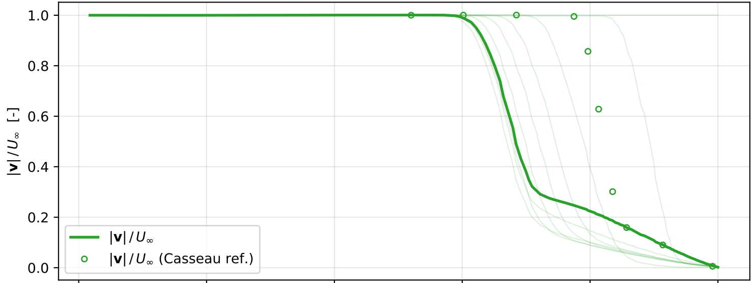
Normalised velocity magnitude
