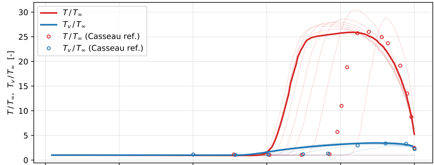
Stagnation-line profiles — t = 1.00\text{e} - 05\text{ s} (faint: 10 equidistant steps) Translational & vibrational temperature
